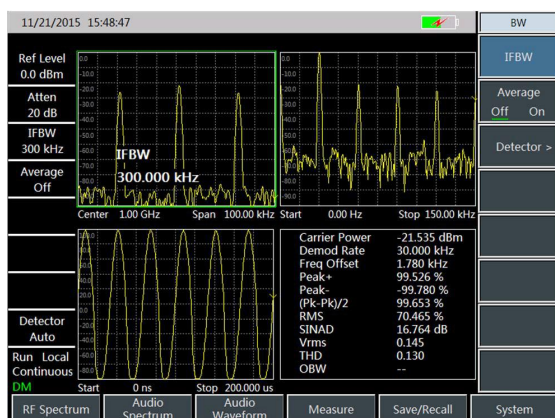
AM/FM/PM Demodulation
